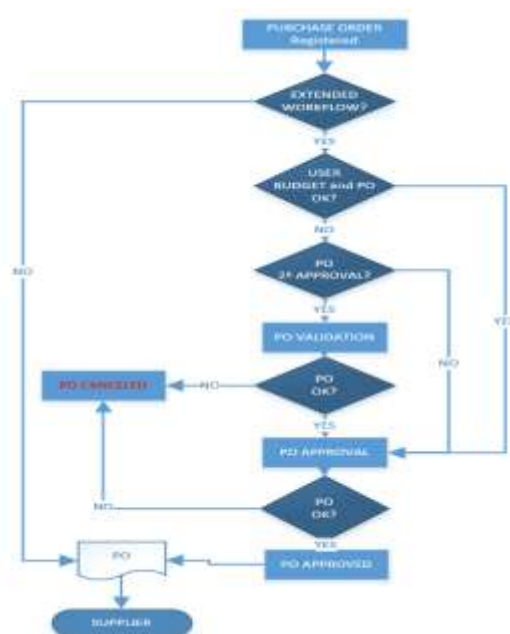
Figure 9 – Purchase orders approval workflow
